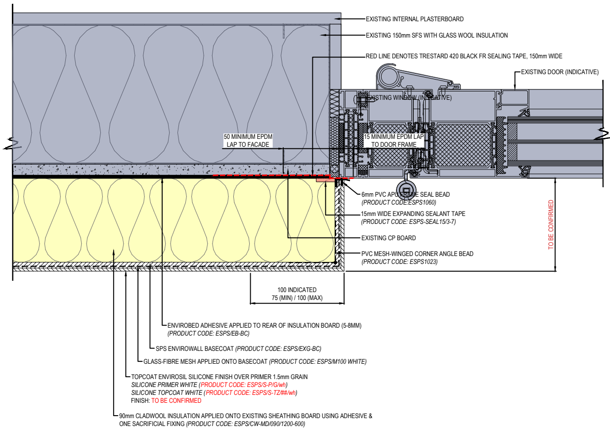
01 PLAN SECTION - RENDER / WINDOW DOOR INTERFACE DETAIL Scale 1:2
