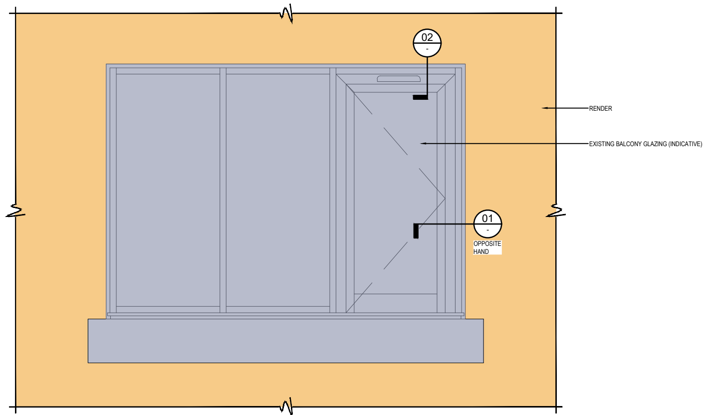
03 PART ELEVATION - RENDER / DOOR JAMB INTERFACE Scale 1:15
