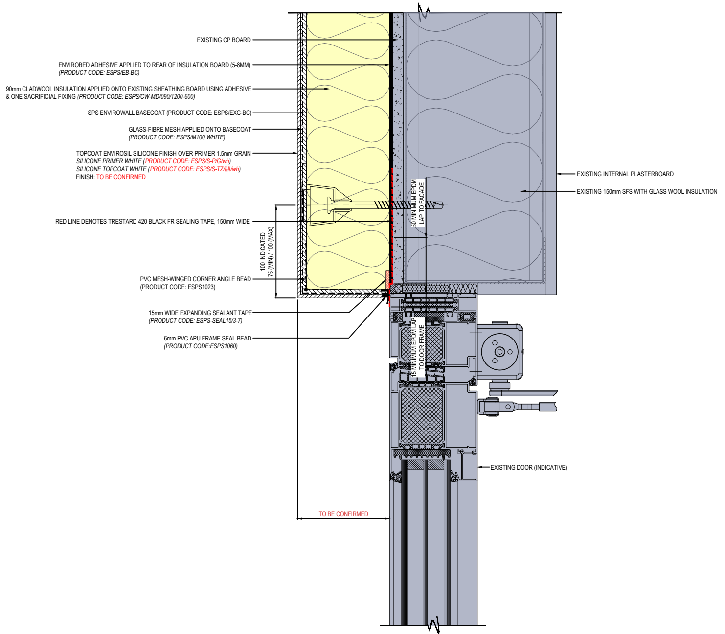
02 CROSS SECTION - RENDER / DOOR HEAD INTERFACE DETAIL Scale 1:2
